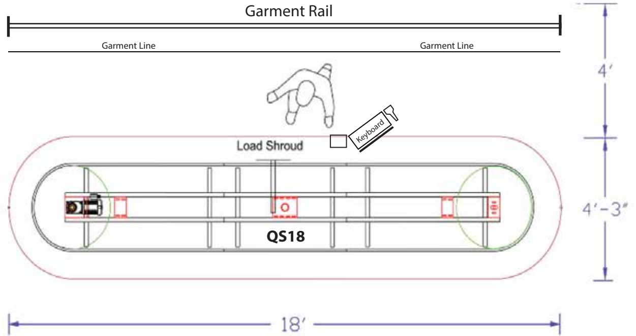
QS18 Typical Layout
